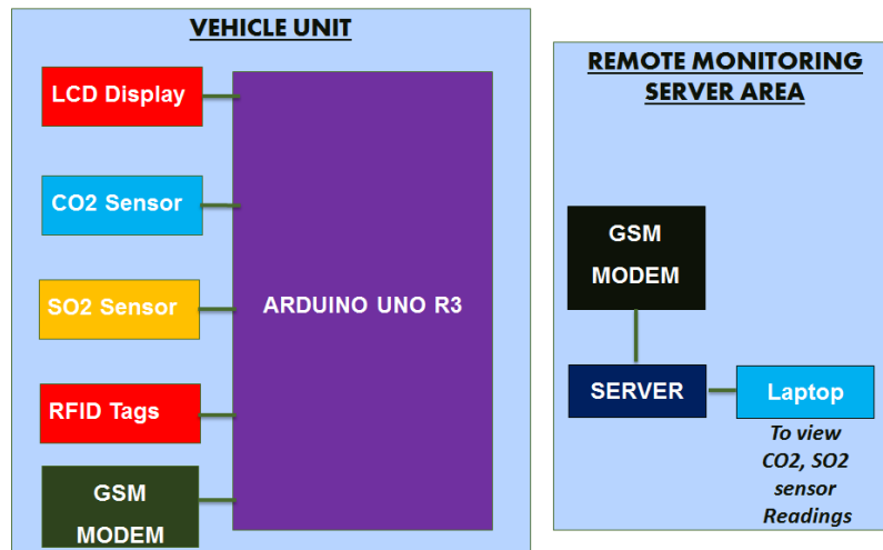
Fig. 1. Block diagram of Vehicular Pollution and Status Monitoring Using IoT
