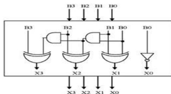
Fig.2: 4-Bit BEC
