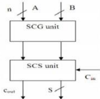
Fig.3.structure of conventional CSLA
