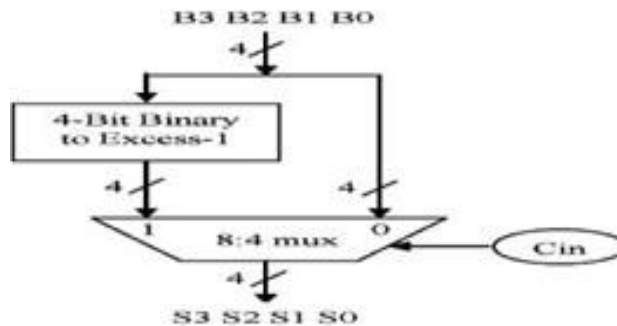
Fig.3: Basic function of the CSLA
