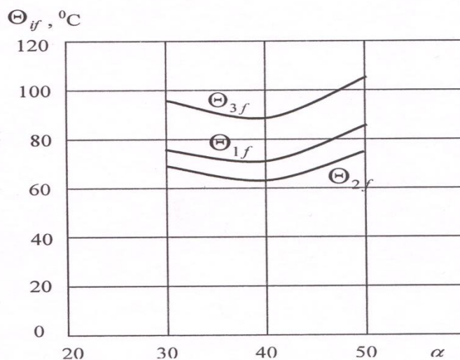
Fig. 4. Changes, exceeding the temperature of thermal bodies of frequency-controlled IM of A4-457-UH-8UZ type in the frequency function
