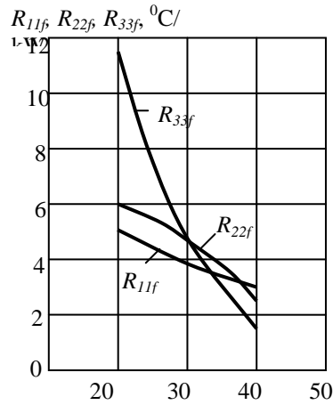
Fig. 1. The change of the total thermal resistances of the thermal bodies of frequency-controlled IM of A4-457-UH-8UZ type in frequency function
