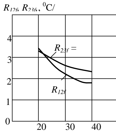
Fig. 2. Changes of the thermal resistances between the thermal bodies of frequency-controlled IM of A4-457-UH-8UZ type in frequency function
