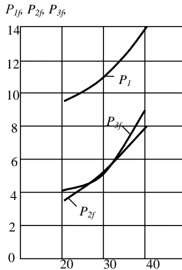
Fig. 3. Changes of the power losses of thermal bodies of frequency-controlled IM of A4-457-UH-8UZ type in frequency function
