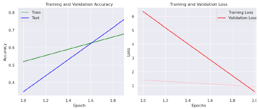
Fig7: Results of Training model
