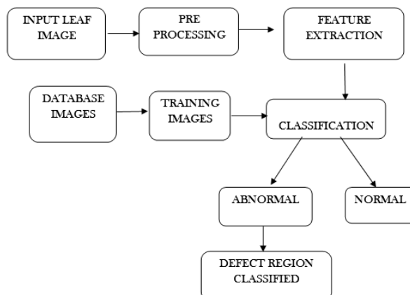
Fig4. Dataflow Diagram
