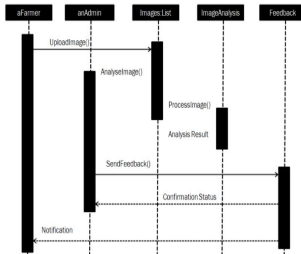
Fig3. Sequence Diagram.
