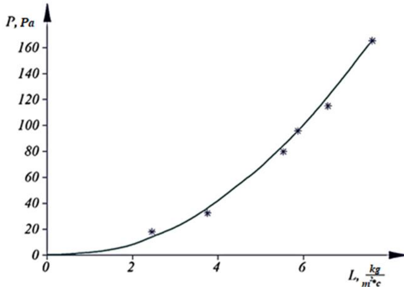
Fig.3.3 Dependence of aerodynamic drag of the nozzle chamber on the mass velocity of the air flow
