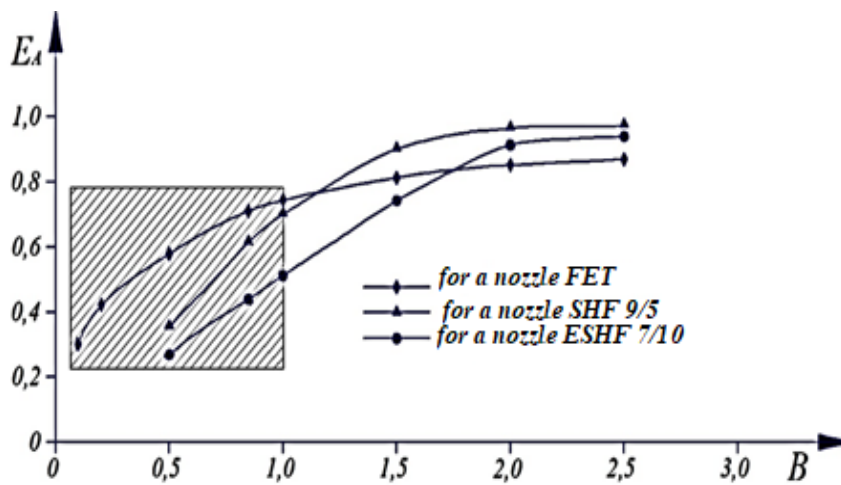
Fig.3.1 Dependence E_A = f(B) for different nozzle types.
