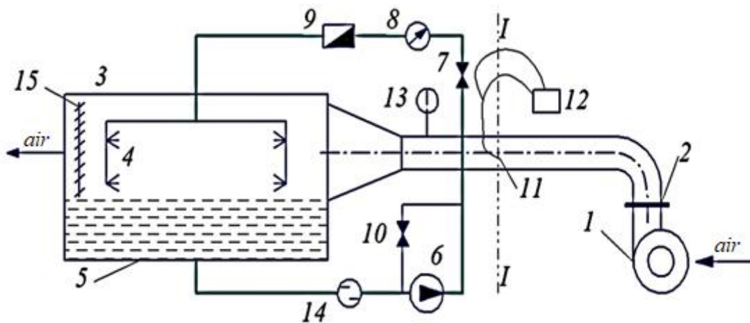
Fig.2.1 Diagram of laboratory installation: 1 - radial fan, 2 - gate valve, 3 - nozzle chamber, 4 - nozzles, 5 - pan, 6 - centrifugal pump, 7 - regulating valve, 8 - manometer, 9 - water meter, 10 - overflow valve, 11 - combined pressure receiver, 12 - micro-manometer, 13 - glass thermometer, 14 - filter, 15 - drift eliminator.
