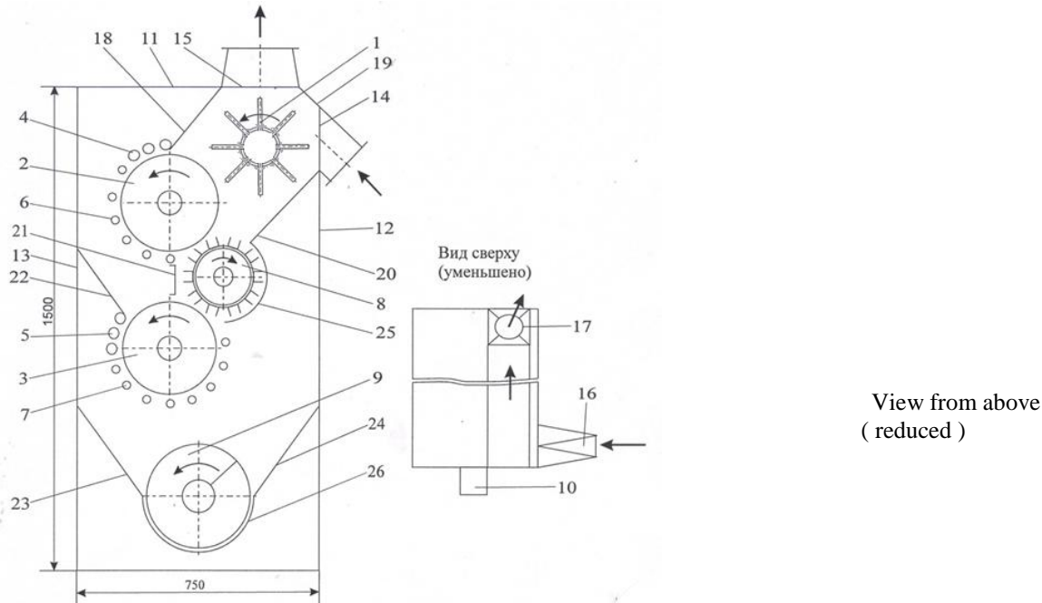
1-bar loosening drum, 2, 3-main and regeneration saw cylinders, 4, 5-fixing grates, 6,7-cleaning grates, 8-slat removing drum, 9-scraper auger, 10-tube with valves, 11- upper cover, 12, 13-front and back wall, 14, 15-inlet and outlet, 16, 17-inlet and outlet, 18,19,20-guard trays, 21-shield, 22, 23, 24-guide trays, 25-guarding casing, 26-trough.
